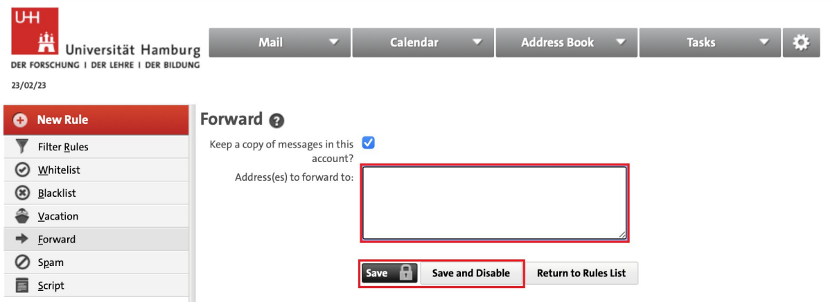
Fig. 6 Forwarding mails
