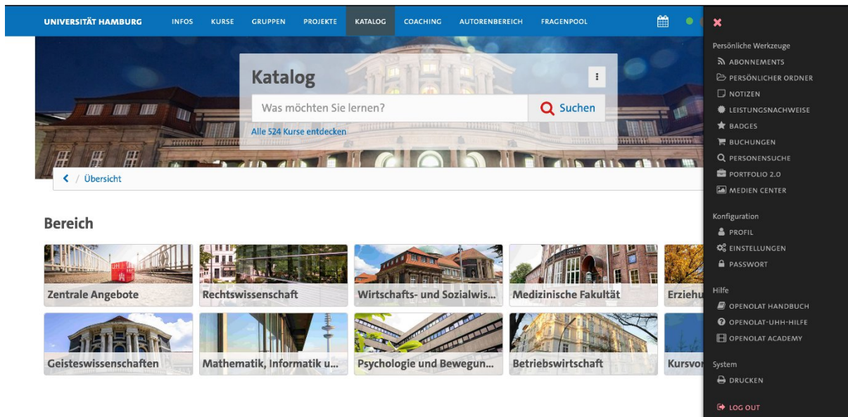
Fig. 10 OpenOlat catalogue
